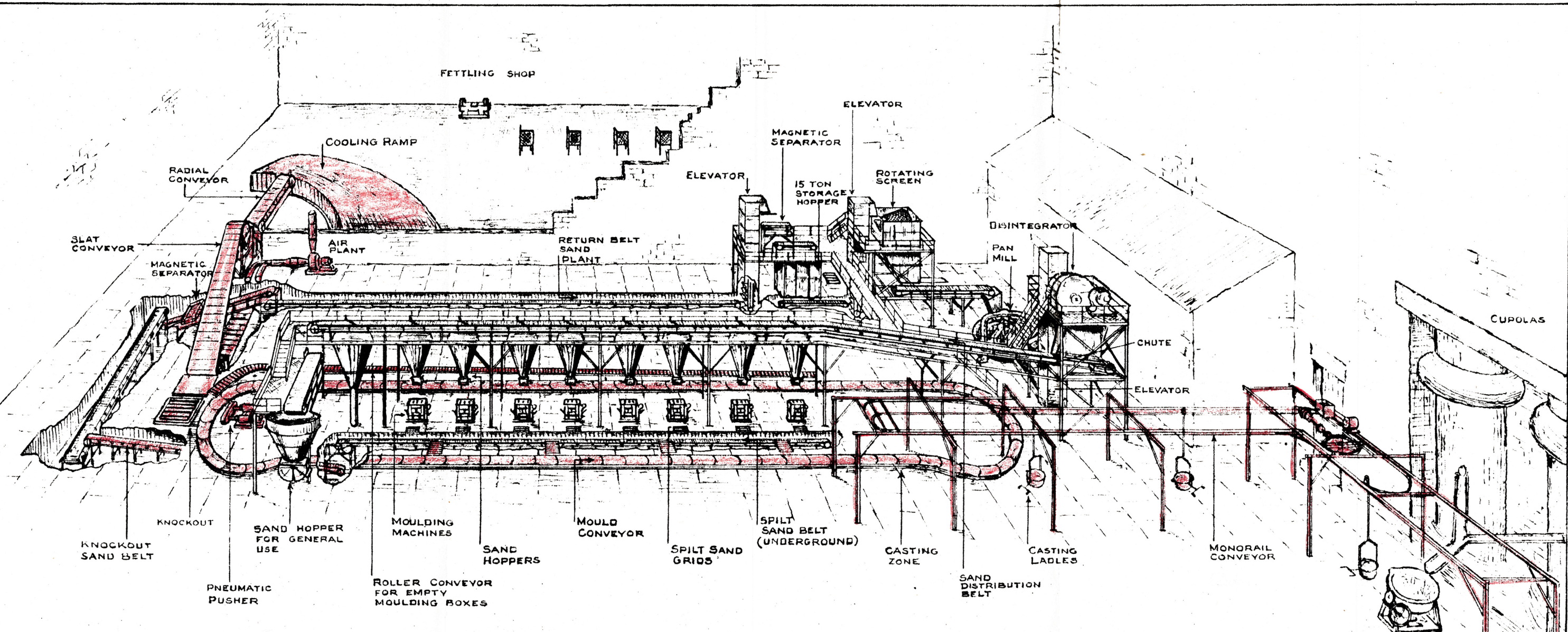
IRON FOUNDRY MECHANIZATION — L M S RLY. ST.ROLLOX
